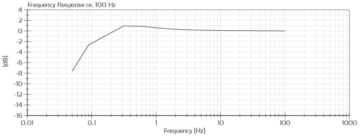
Typical frequency response below 250 Hz
