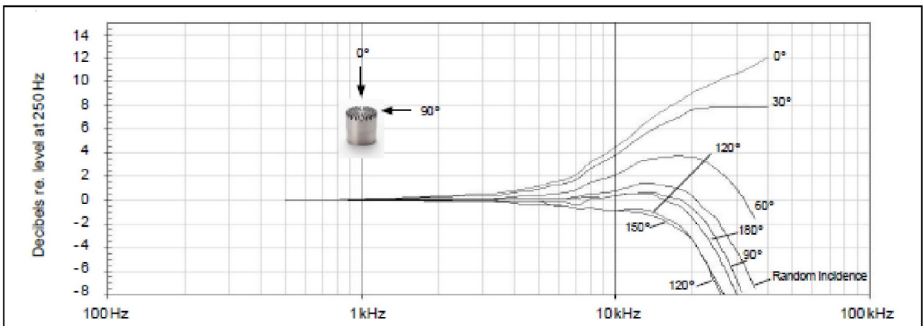
Free-field corrections for various degrees of incidence
